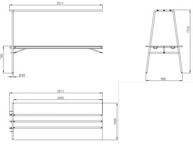
FourReal A XL Extension H740xL2400xW1000
