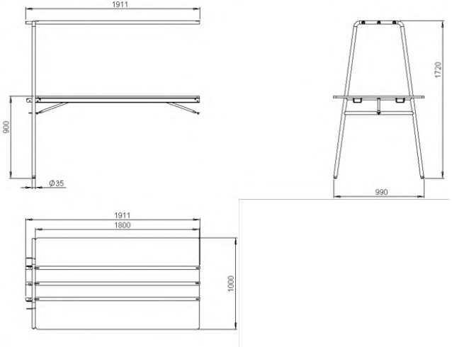
FourReal A XL Extension H900xL1800xW1000
