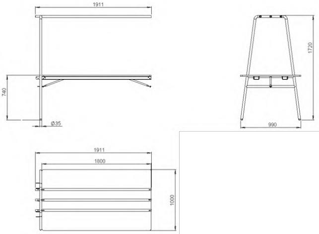
FourReal A XL Extension H740xL1800xW1000
